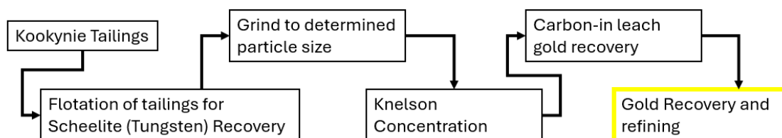
Figure 2: Proposed further metallurgical test work flowsheet designed to validate and optimise the processing circuit.
