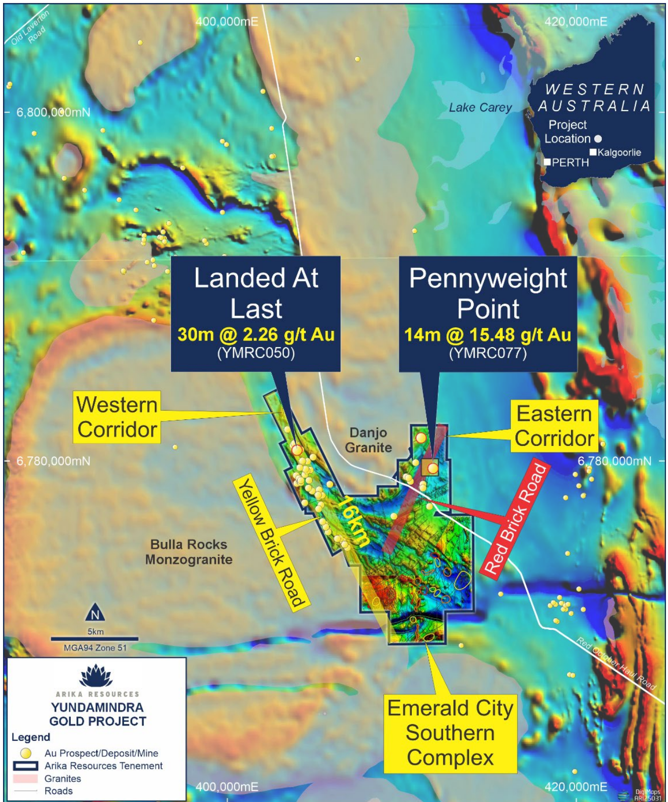
Figure 5: Yundamindra Gold Project regional setting showing key target areas and prospects over detailed project TMI and regional TMI.
