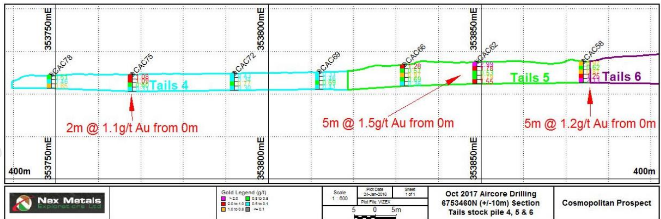
Figure 2. 6753430N Cross section (+/-10) showing aircore drilling across Cosmopolitan stockpiles 4, 5 & 6.
